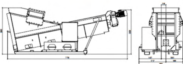
Transport positie
